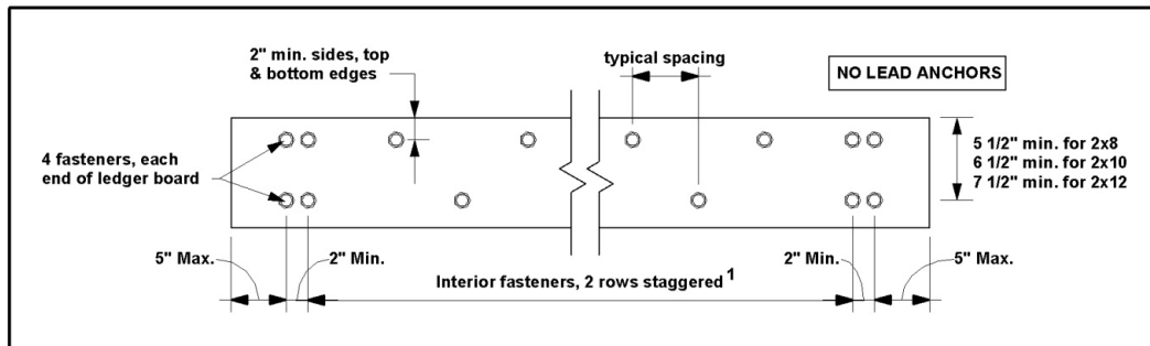
FIGURE 20: LEDGER BOARD FASTENER SPACING AND CLEARANCES
