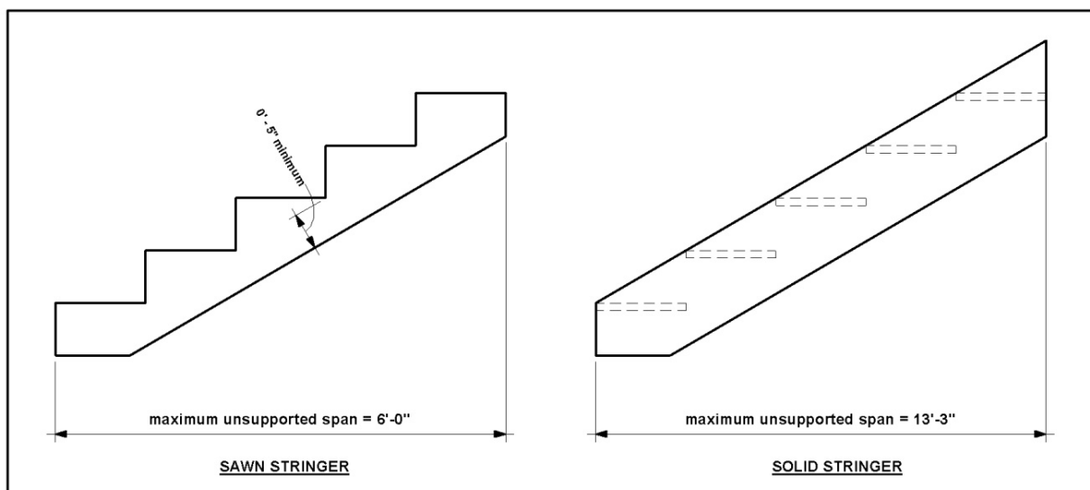
FIGURE 33: STAIR STRINGER REQUIREMENTS
