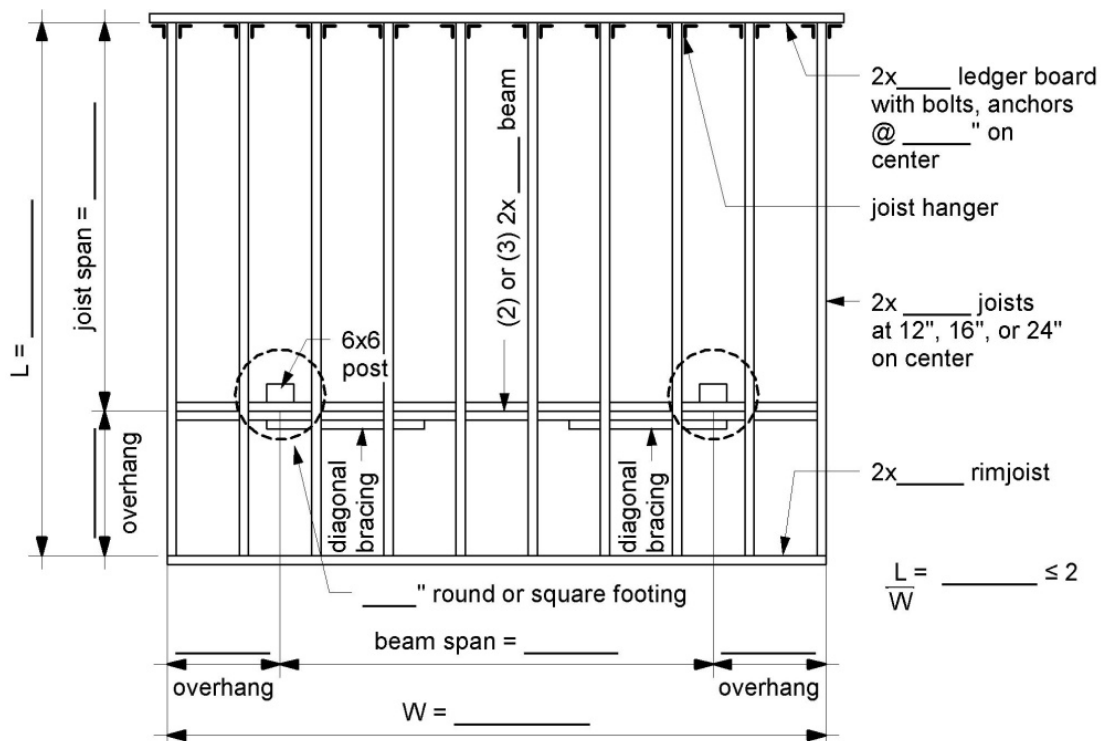
FIGURE 7: TYPICAL DECK FRAMING PLAN
